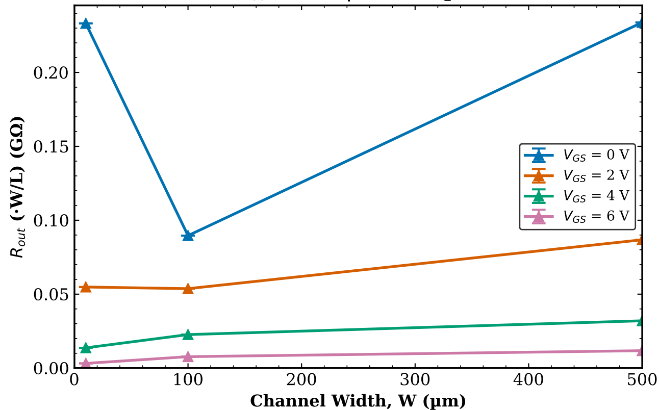
TFT1 Transistor 1 R_{out} vs W | L = 20\text{ }\mu\text{m}
